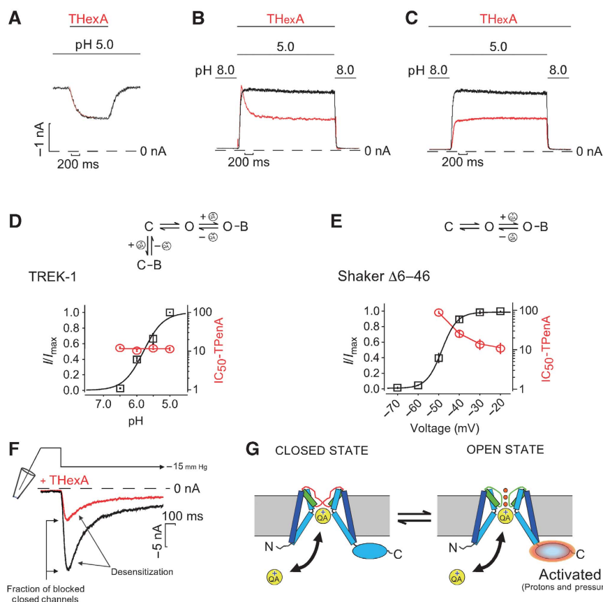
Figure 6 pH activation of TREK-1 does not involve the bundle crossing. (A) TREK currents activated by pH 5 during fast application and wash out of 1 μM THexA. (B) Closed channels at pH 8 were switched into a solution containing 1 μM THexA at pH 5 (red trace) and back to pH 8 showing fast pH-mediated opening and relatively slow blocking by THexA. (C) 1 μM THexA is continuously present during the switch from pH 8 to pH 5 (red trace) and the current is already pre-blocked to 50%, no slow block is observed. (D) As the Po for TREK-1 is increased by acidification to saturating levels no change in IC 50 for TPenA inhibition is observed ( n \geq 6 for each pH). (E) In contrast, in Shaker Δ6-46 channels the IC 50 for TPenA inhibition decreases as relative current increases with voltage activation ( n \geq 4 for each voltage). (F) Pressure activation by 15 mm Hg in absence (black trace) and presence of 1 μM THexA (red trace). (G) TREK-1-gating model. Large movements of the C-terminal regulatory domain are translated into small movements of TM helices to gate the channel at the filter and do not involve gating at the helix bundle crossing.
