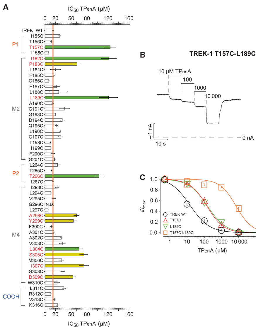
Figure 3 Identification of residues in the TREK-1 pore that affect TPEnA block. (A) IC 50 values of TPEnA inhibition for TREK-1 WT ( n = 11 ) channels and indicated mutations ( n \geq 4 ). The orange line represents the deviation (s.e.m.) of the IC 50 observed for WT channels. Green bars represent mutations thought to contribute directly to the QA binding site and in yellow those mutations which are not part of the binding site. (B) Current trace from the TREK T157C-L189C double mutation that results in a strongly decreased TPEnA affinity. (C) Dose-response relationship from experiments such as in (B) fitted to a standard Hill equation for TREK WT, T157C and L189C mutations and the double mutant which dramatically reduces TPEnA affinity; IC 50 values of 13 \pm 1 , 123 \pm 11 , 120 \pm 18 and 8149 \pm 428 \mu\text{M} for WT ( n = 10 ), T157C ( n = 5 ), L189C ( n = 6 ) and T157C-L189C ( n = 4 ), respectively.
