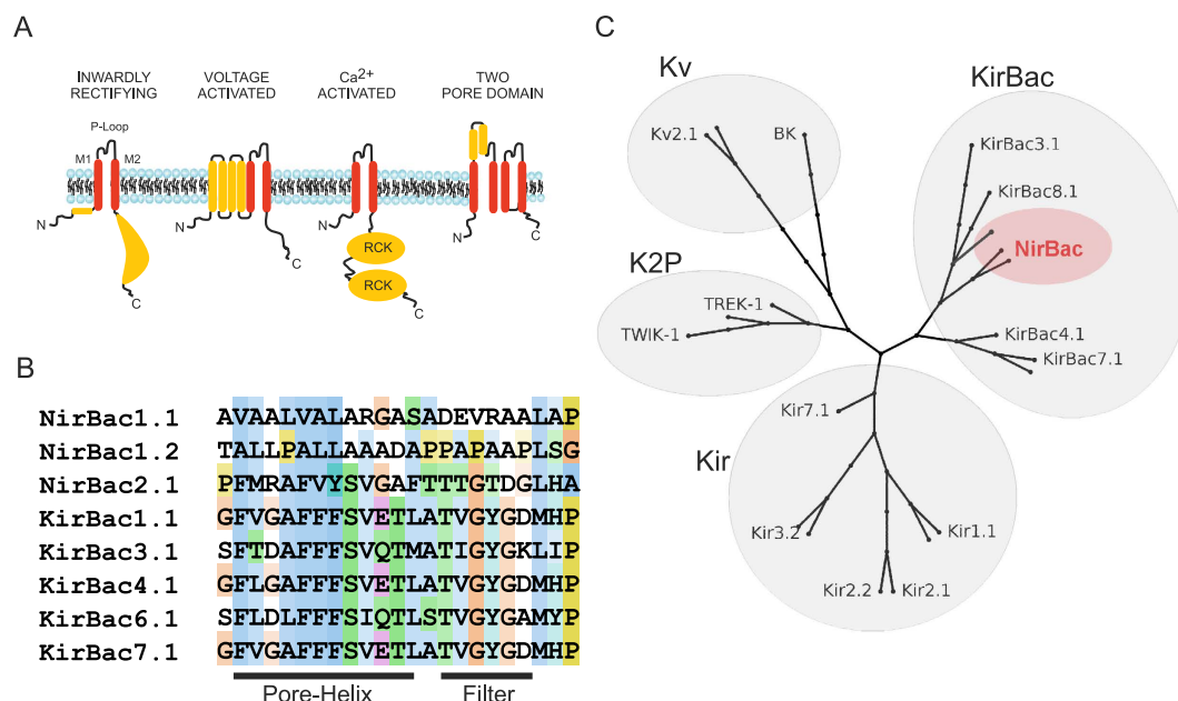
Figure 1. Evolution and modular design of \text{K}^+ channel structures. (A) All \text{K}^+ channels share a conserved P-loop region, which contains the selectivity filter and TM domains which provide passageway through the membrane. These conserved domains can be found fused to a number of different regulatory domains which results in a number of functionally different \text{K}^+ channel families, including the inward rectifiers (Kir), voltage gated channels (Kv), calcium activated channels and Two-Pore channels (K2P). (B) An alignment of the P-loop regions of prokaryotic Kir channel homologues, KirBac, with the P-loop sequences of the novel inwardly rectifying channels, NirBac1.1, NirBac1.2 and NirBac2.1. (C) A phylogenetic tree showing that NirBac channels are placed firmly in the family of prokaryotic inward rectifiers.
