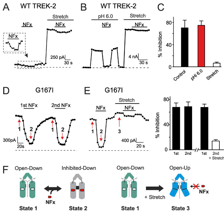
Figure 2. Dynamic interconversion between structurally distinct open conformations. (A) Example showing WT TREK-2 currents from an inside-out patch; at pH i 7.4, channels can be inhibited by 10 μM NFX (effect magnified within inset dashed box). Channels were then stretch activated by application of negative pressure (−11 mmHg suction to the pipette), whereupon NFX inhibition is markedly reduced. Currents were recorded from voltage steps to 0 mV from a holding potential of −80 mV. The dashed line indicates the zero current level. (B) Similar dynamic changes in NFX inhibition can also be observed for channels activated by intracellular acidification (pH i 6.0), demonstrating that these two activated states are structurally distinct. (C) Summary of dynamic changes in NFX inhibition seen for stretch activation but not pH i activation. (D) Repeated NFX application produces consistent inhibition of the G167I mutant channel. The red arrows indicate distinct structural states of the channel. (E) Example experiment (similar to that shown in A and B) showing a dynamic change in NFX inhibition for the G167I mutant as the channel is converted from the down state to the up by membrane stretch. (C and E) Error bars shown are mean ± SEM ( n \geq 6 ). (F) Cartoon illustrating conversion between
