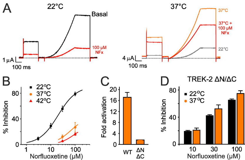
Figure 4. Temperature activation involves conformational changes in the TM helices. (A) Example traces showing that temperature-dependent activation of whole-cell TREK-2 currents from 22^\circ C (left) to 37^\circ C (right) markedly decreases inhibition by 100 \mu M NFX. For comparison, the currents at 22^\circ C are also shown in gray in the right panel. Currents were recorded by voltage protocols similar to those used in Fig. 1 D. (B) Summary dose-response curves showing reduced NFX sensitivity of whole-cell TREK-2 currents at 22^\circ C , 37^\circ C , and 42^\circ C (data shown are percent inhibition of basal currents recorded at 0 mV ; mean \pm SEM, n \geq 6 ). IC_{50} at 22^\circ C , 23.4 \pm 3.1 \mu M ; but at 37^\circ C and 42^\circ C , >100 \mu M . (C) A truncated version of TREK-2 (TREK2 \Delta N/\Delta C ) that no longer responds to temperature. Fold activation represents change in current between 22^\circ C and 37^\circ C . (D) The NFX sensitivity of this temperature-insensitive mutant is unaffected by temperature, indicating a specific effect on WT TREK-2. (C and D) Error bars shown are mean \pm SEM ( n \geq 6 ).
